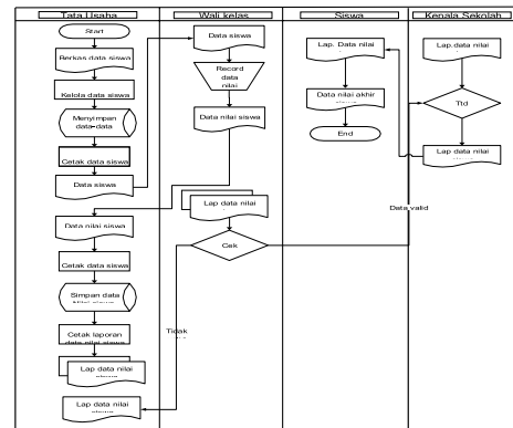
Rancangan flowchart
